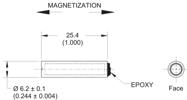
ALNICO 8 MAGNET, VALOX 420 SEO CAPSULE
