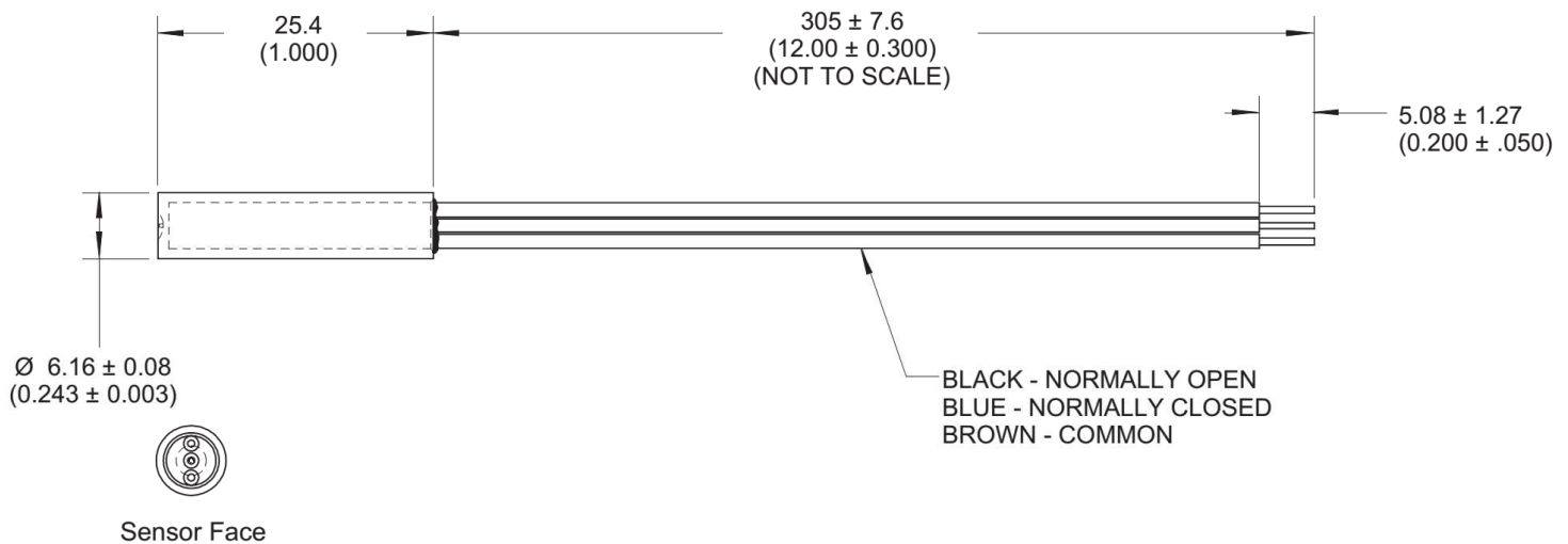
MAGNETIC ACTUATOR AS201701
