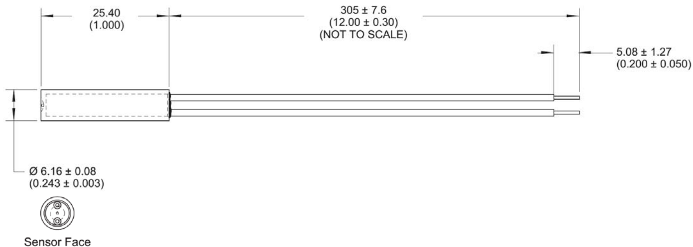
MP201703 (Form C - SPDT Changeover)
