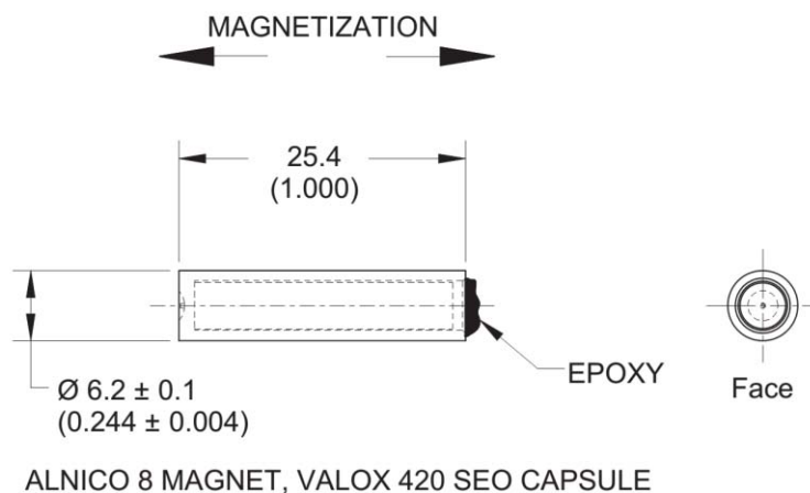
MAGNETIC ACTUATOR AS201701
