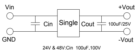
Recommended Test Circuit
