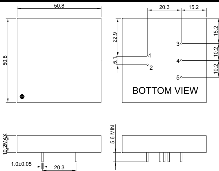
Markings and dimensions
