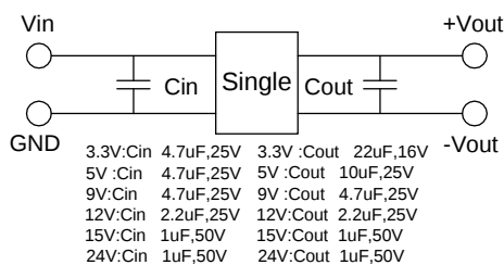
Recommended Test Circuit
