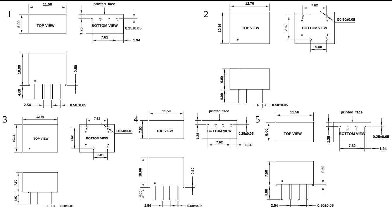
Markings and dimensions
