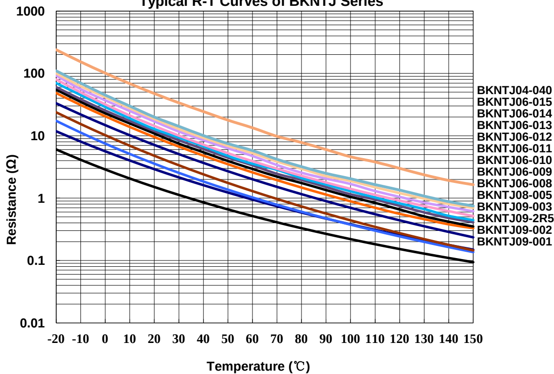
Typical R-T Curves of BKNTJ Series
