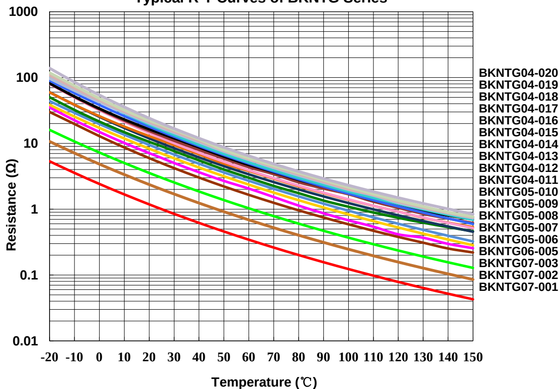
Typical R-T Curves of BKNTG Series
