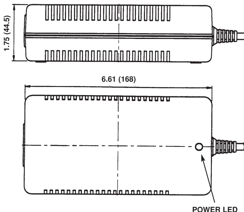
POWER LED
