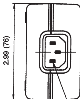
AC INPUT IEC 320 INLET
