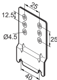
Mounting plate for units with hood
