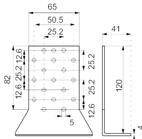
Univ. mounting bracket
