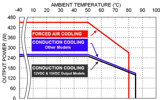
Derating Curve vs. Ambient Temperature Vin=115VAC and Forced Air Cooling (Internal Fan) Top & Side Fan Models
