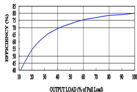
LANEUW2405R3 Efficiency vs Output Load
