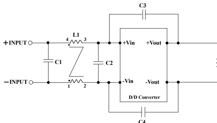
Recommended Filter for EN55022 Class B Compliance
