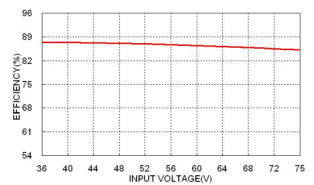
JFCW48S33-30 Efficiency vs. Input Voltage, Full Load
