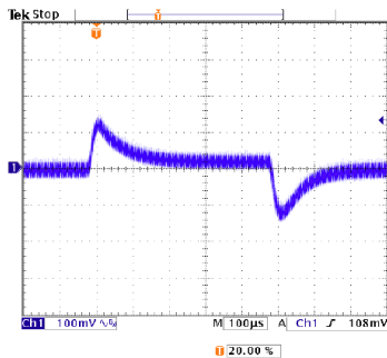
JFCW24S05-30 Transient Response to Dynamic Load Change from 100% to 75% to 100% of Full Load; Vin (nom)
