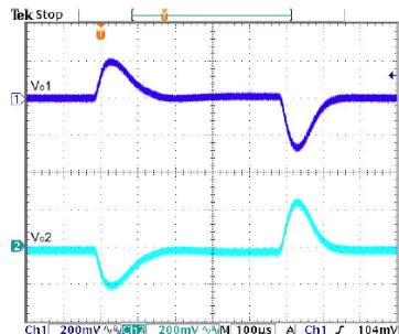
JFCW48D12-30 Transient Response to Dynamic Load Change from 100% to 75% to 100% of Full Load; Vin (nom)
