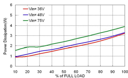
JFCW48S33-30 Power Dissipation vs. Output Load
