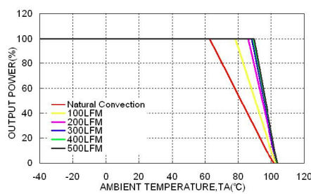
JFCW24S12-30 Derating Output Load vs. Ambient Temperature with Heatsink and Airflow, Vin (nom)
