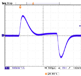
JFCW48S12-30 Transient Response to Dynamic Load Change from 100% to 75% to 100% of Full Load; Vin (nom)
