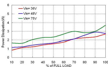
JFCW48D24-30 Power Dissipation vs. Output Load
