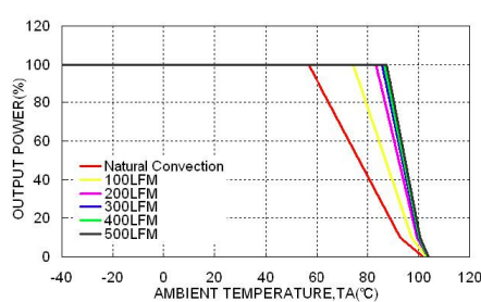
JFCW24S33-30 Derating Output Load vs. Ambient Temperature with Heatsink and Airflow, Vin (nom)
