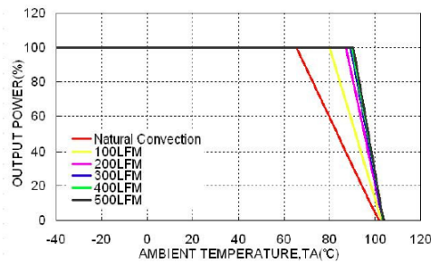
Ambient Temperature with Heatsink and Airflow, Vin (nom)
