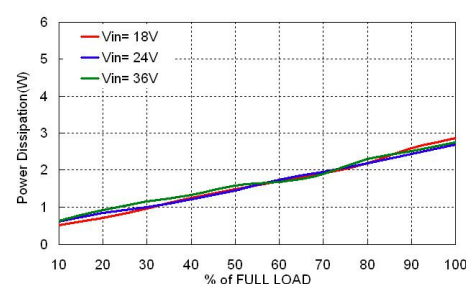
JFCW24S15-30 Power Dissipation vs. Output Load
