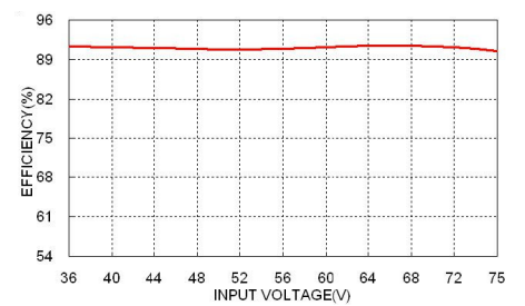
JFCW48S15-30 Efficiency vs. Input Voltage, Full Load
