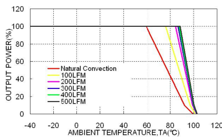
JFCW48S33-30 Derating Output Load vs. Ambient Temperature with Heatsink and Airflow, Vin (nom)
