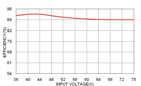
JFCW48D24-30 Efficiency vs. Input Voltage, Full Load
