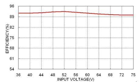
JFCW48S24-30 Efficiency vs. Input Voltage, Full Load
