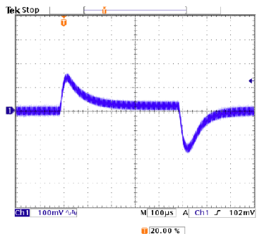
JFCW48S05-30 Transient Response to Dynamic Load Change from 100% to 75% to 100% of Full Load; Vin (nom)
