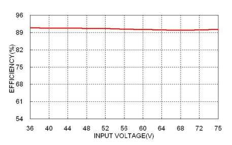
JFCW48S12-30 Efficiency vs. Input Voltage, Full Load
