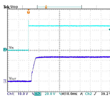
JFCW48S24-30 Typical Input Start-Up and Output Rise Characteristic Vin (nom); Full Load
