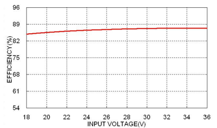
JFCW24S33-30 Efficiency vs. Input Voltage, Full Load
