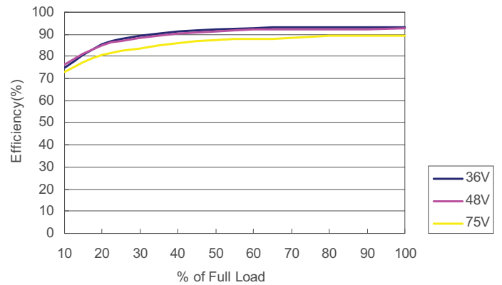
DH48S15-40 Efficiency vs Load Current
