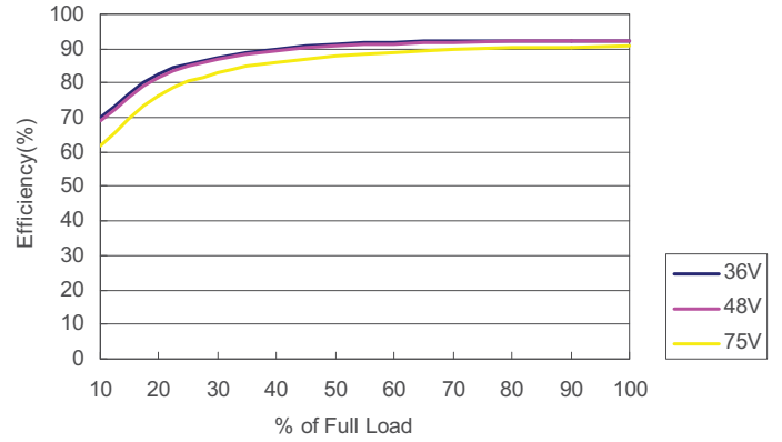
DH48S5-40 Efficiency vs Load Current
