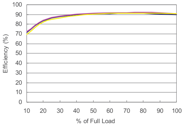
DH12S3.3-26 Efficiency vs Load Current
