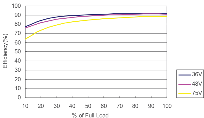
DH48D12-40 Efficiency vs Load Current
