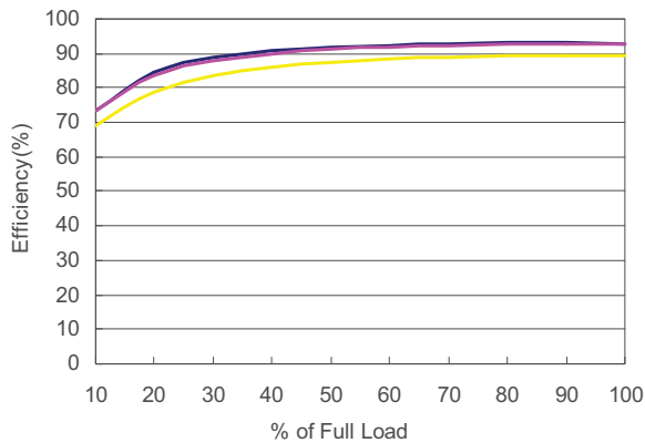
DH24S12-40 Efficiency vs Load Current
