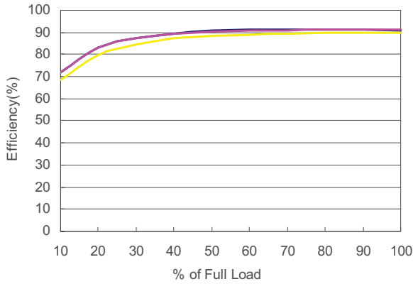
DH24S3.3-26 Efficiency vs Load Current
