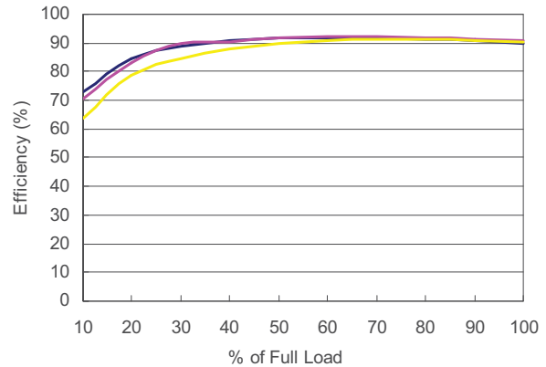
DH12S5-40 Efficiency vs Load Current
