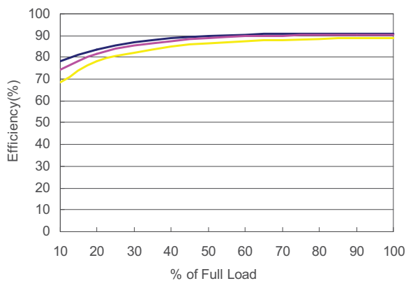
DH24D12-40 Efficiency vs Load Current
