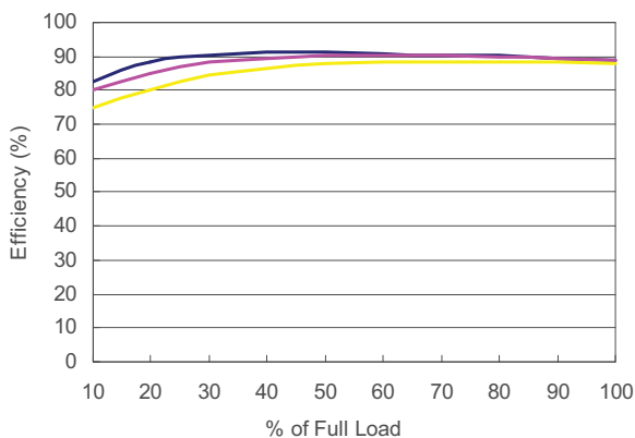
DH12D12-40 Efficiency vs Load Current
