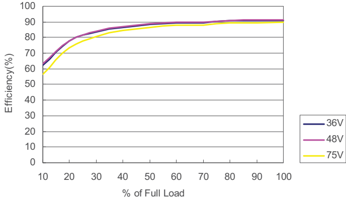
DH48S3.3-26 Efficiency vs Load Current
