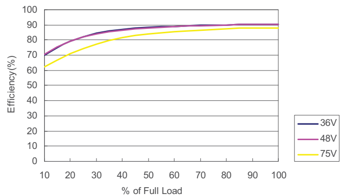
DH48D15-40 Efficiency vs Load Current
