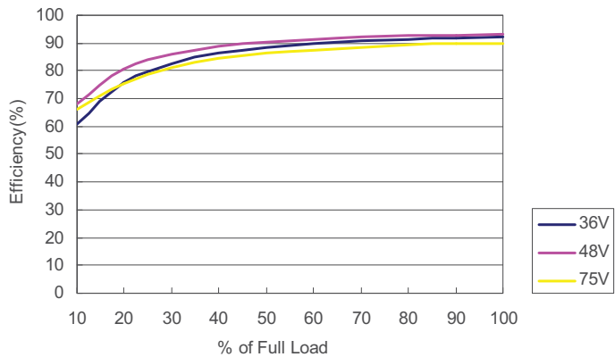
DH48S12-40 Efficiency vs Load Current
