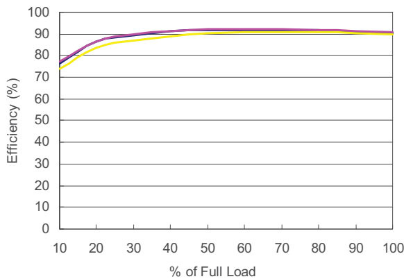
DH12S12-40 Efficiency vs Load Current
