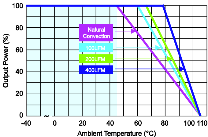
DH12S12-50, DH12S15-50, DH12S24-50, DH24S24-50, DH48S24-50 Derating Curve Without Heatsink
