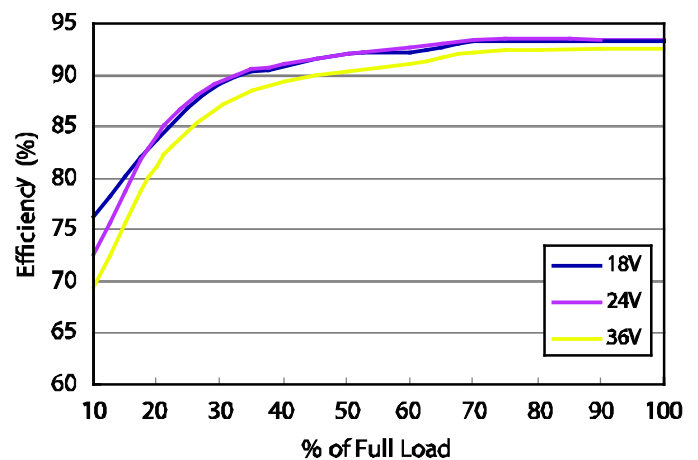
DH24S12-50 Efficiency vs Load Current
