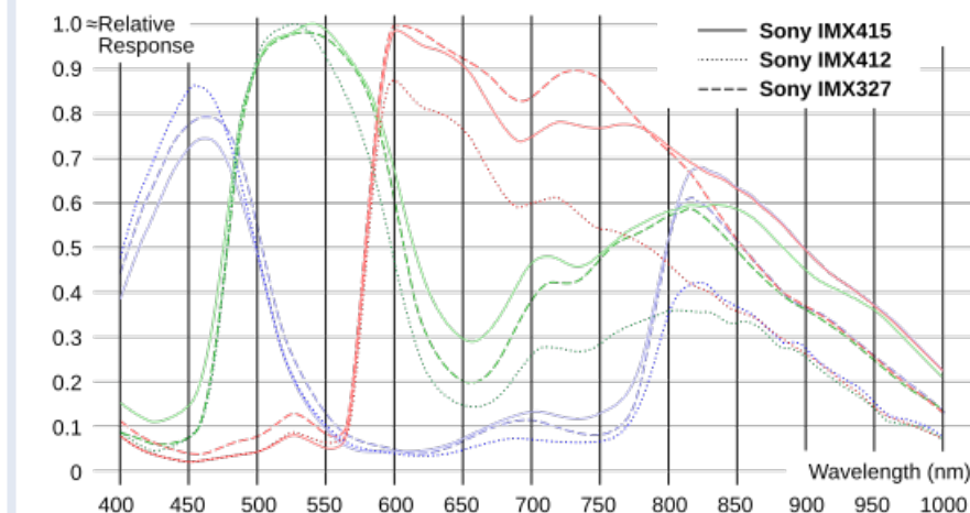
Spectral Curves of selected Color Sensors (1)
