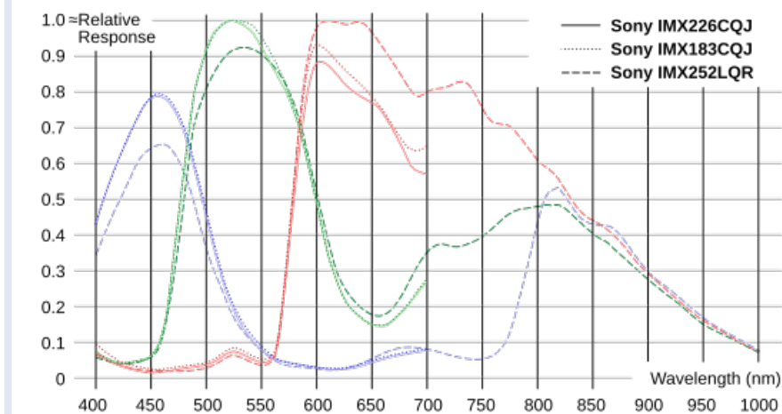
Spectral Curves of selected Color Sensors (2)
