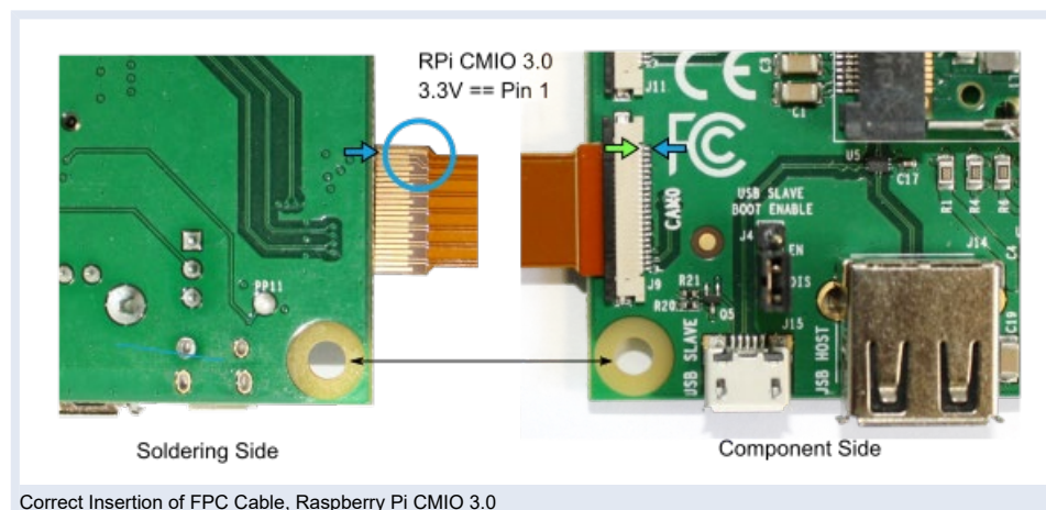
Correct Insertion of FPC Cable, Raspberry Pi CMIO 3.0
