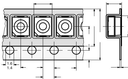
Fig. 11 - Tape Dimensions in mm for PLCC-2
