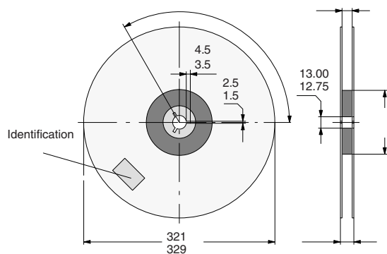
Fig. 15 - Dimensions of Reel-GS18
