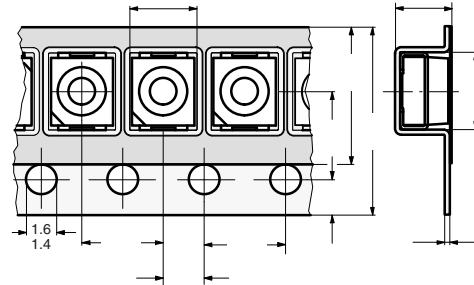
Fig. 12 - Tape Dimensions in mm for PLCC-3
