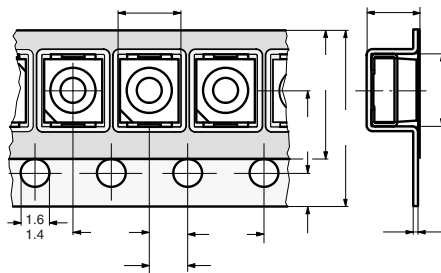
Fig. 12 - Tape Dimensions in mm for PLCC-2
