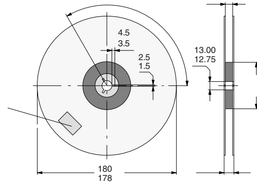
Fig. 14 - Dimensions of Reel-GS08
