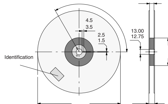
Fig. 15 - Dimensions of Reel-GS18
