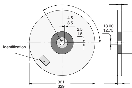
Fig. 15 - Dimensions of Reel-GS18
