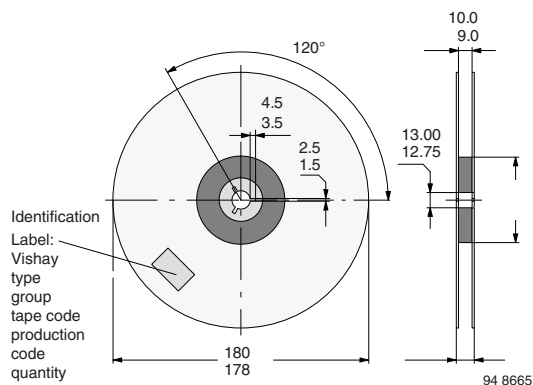
Fig. 14 - Dimensions of Reel-GS08
