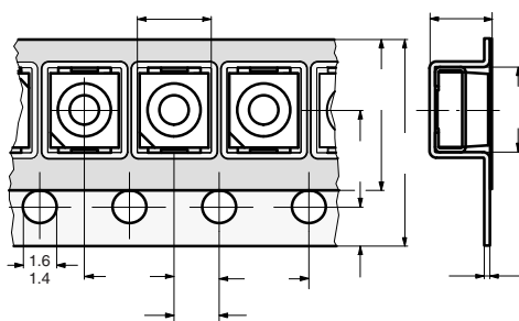
Fig. 12 - Tape Dimensions in mm for PLCC-2
