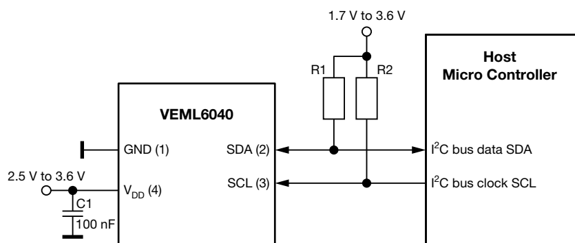
Fig. 7 - Hardware Pin Connection Diagram
