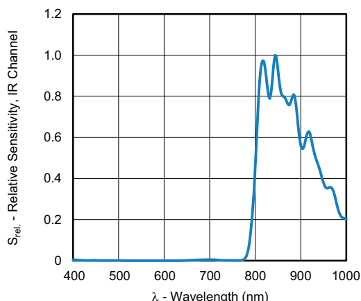
Fig. 6 - Relative Sensitivity, IR Channel vs. Wavelength
