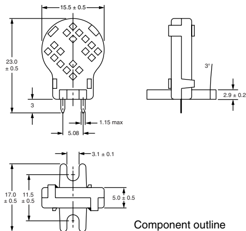
Component outline
