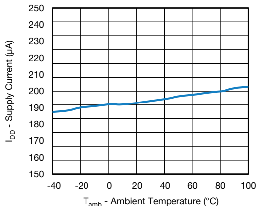
Fig. 6 - Supply Current vs. Ambient Temperature
