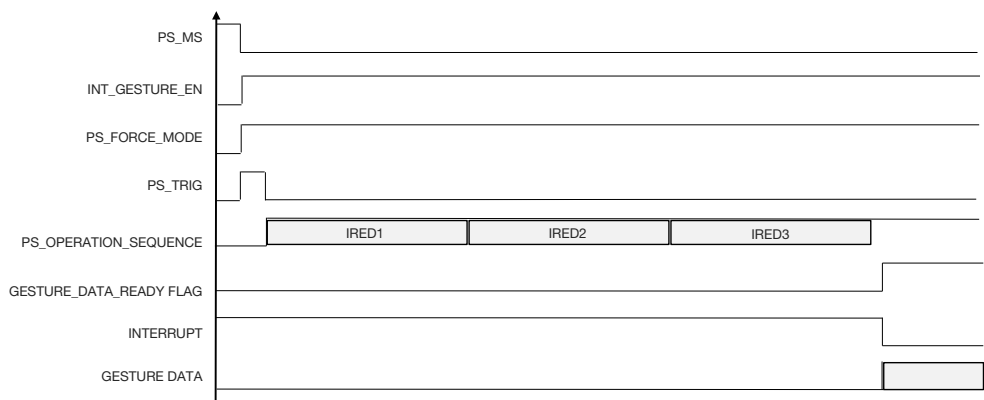
Fig. 11 - VC�L4035X01 Gesture Mode Sequence
