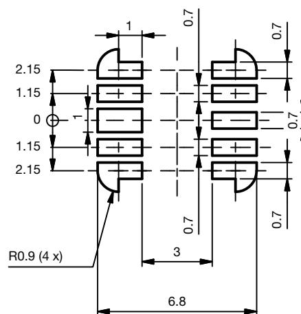
Recommended Footprint
