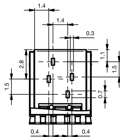
Recommended Footprint
