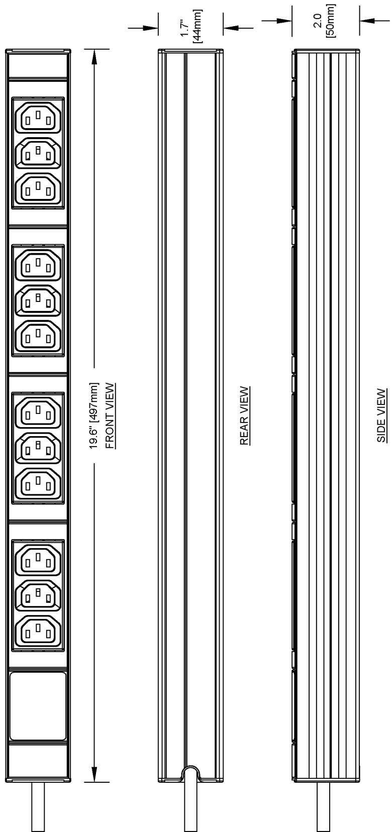
Figure 10 Knurr DI-STRIP 35352031
