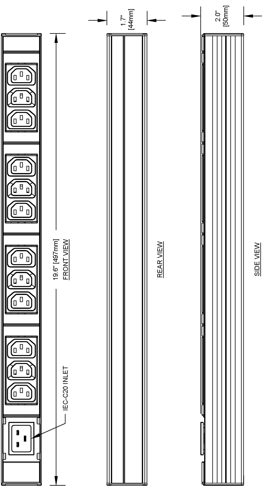
Figure 11 Knurr DI-STRIP 35352041
