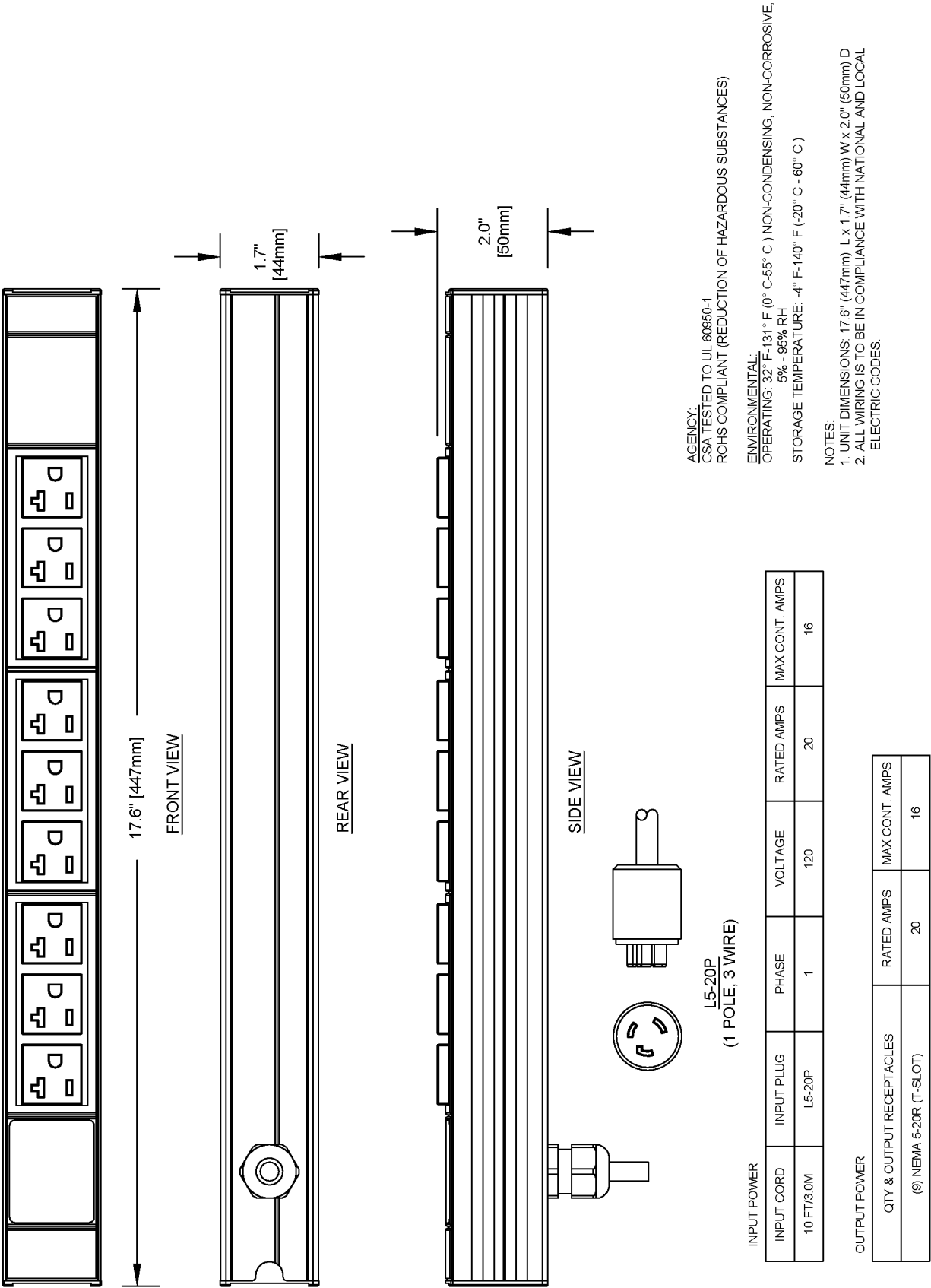
Figure 4 Knurr DI-STRIP 35351041
