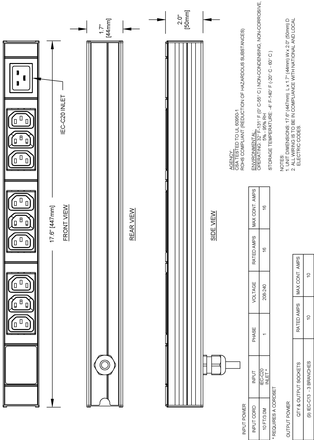
Figure 9 Knurr DI-STRIP 35352021
