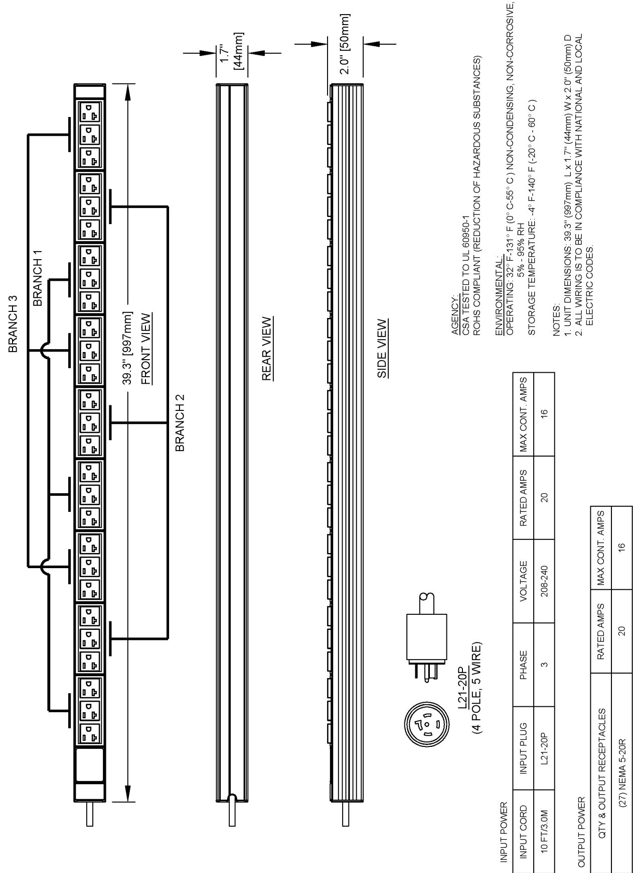
Figure 18 Knurr DI-STRIP 35353041
