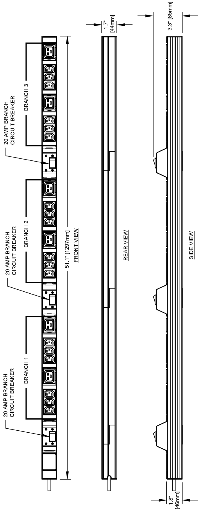
Figure 19 Knurr DI-STRIP 35353051
