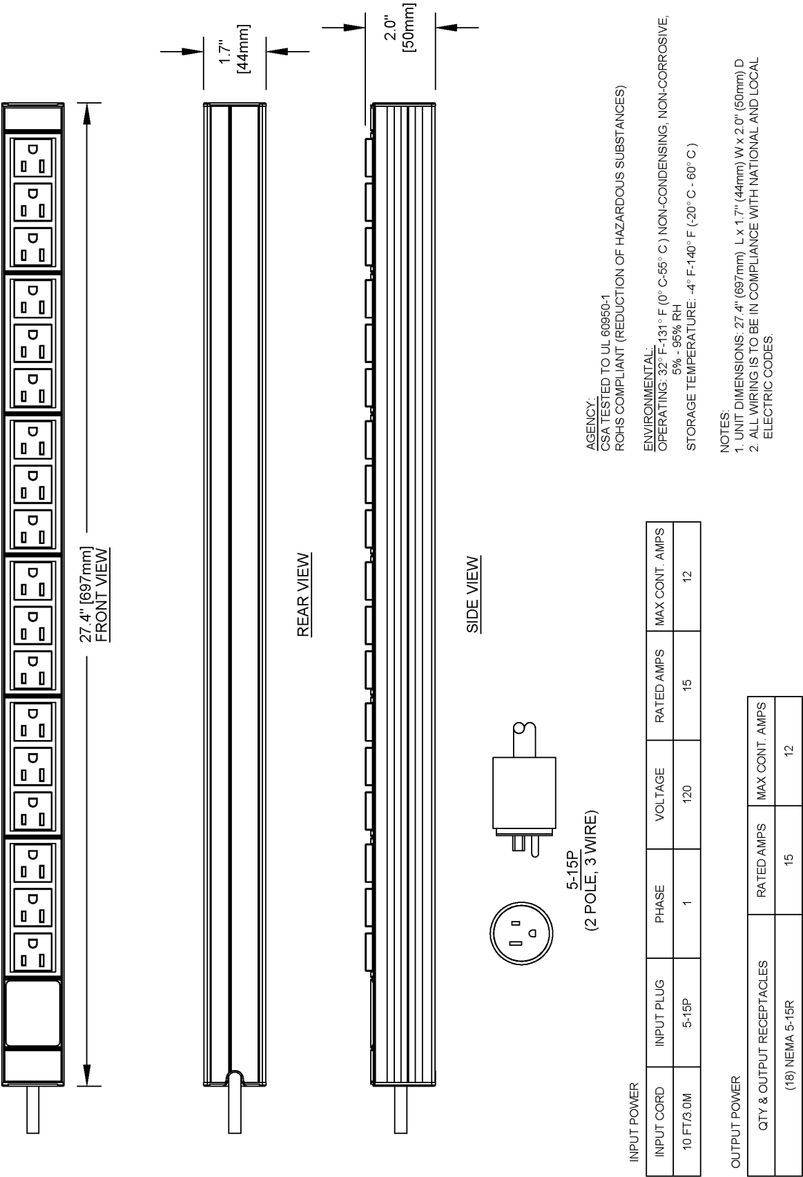
Figure 3 Knurr DI-STRIP 35351031
