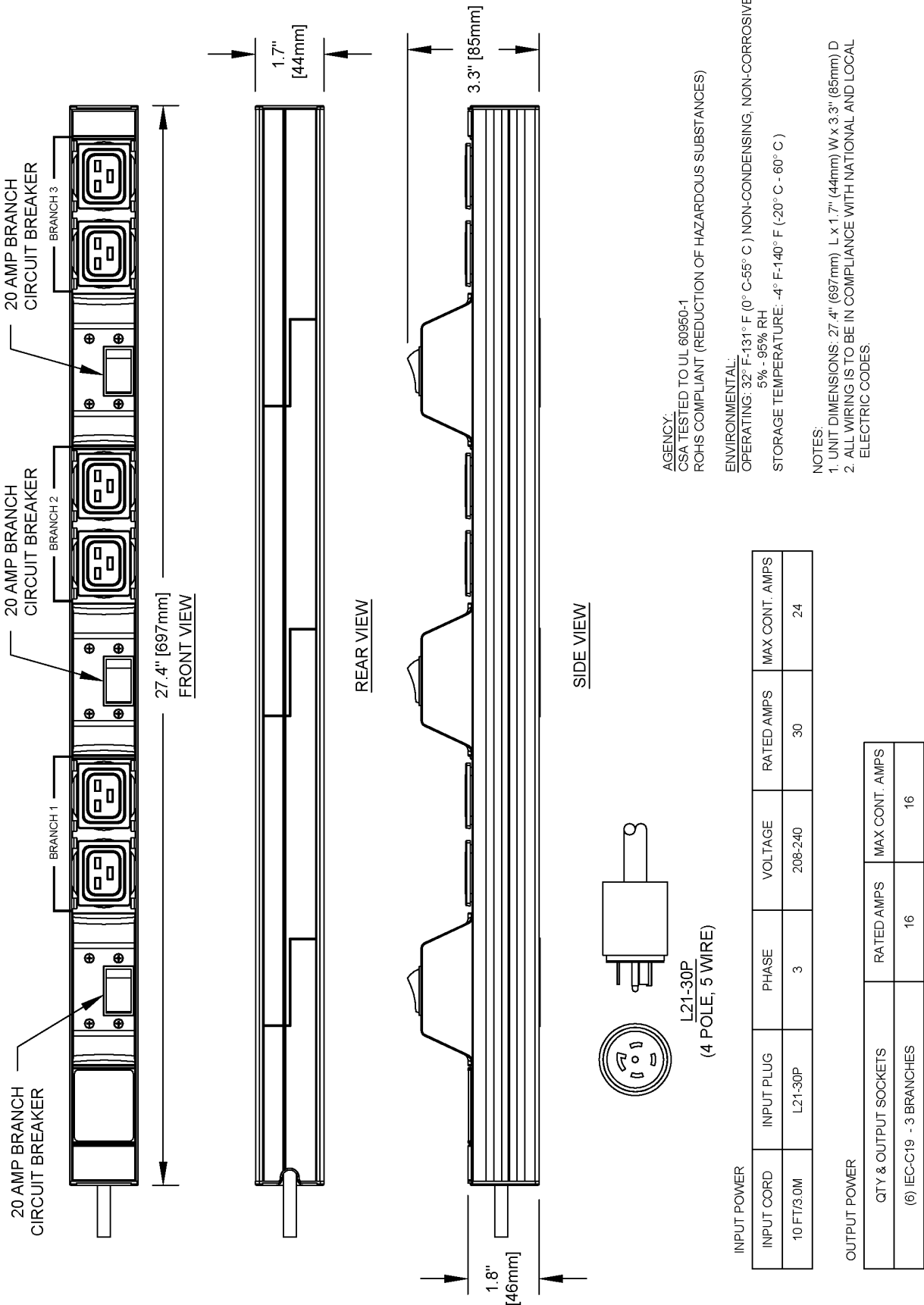
Figure 15 Knurr DI-STRIP 35353011
