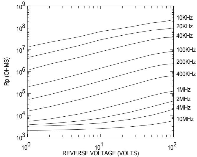
TYPICAL Rp vs REVERSE VOLTAGE
