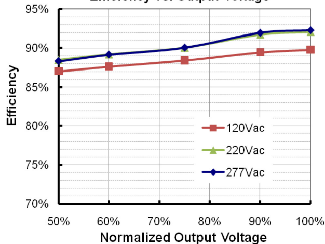
PIL150BU-C3150-DT/ST Efficiency vs. Output Voltage
