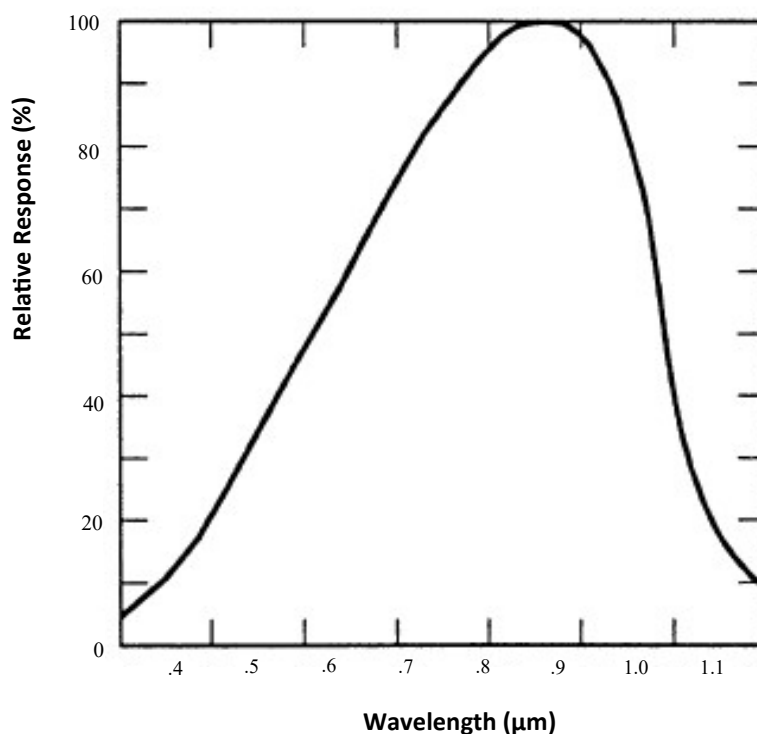
Spectral Responsivity
