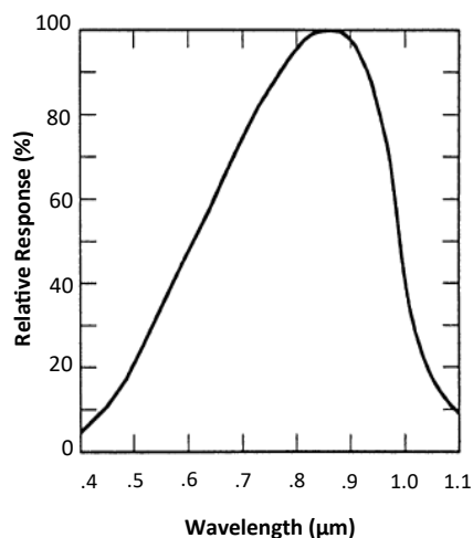
Spectral Responsivity
