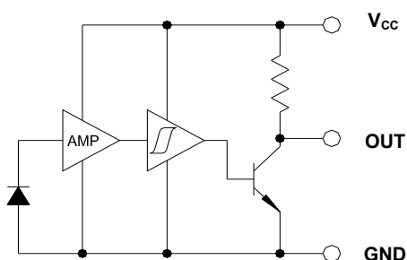
OPL530/535A/535B 10 K Pull-Up
