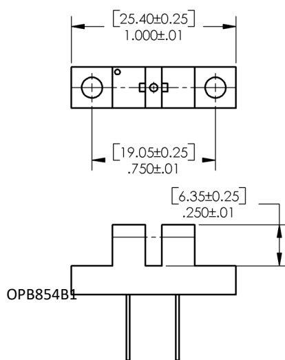
OPB854A3/OPB854B3 - Housing
