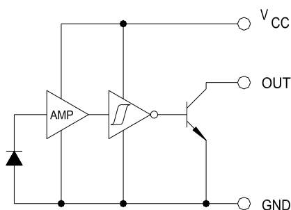
OPB698 Inverted Open-Collector
