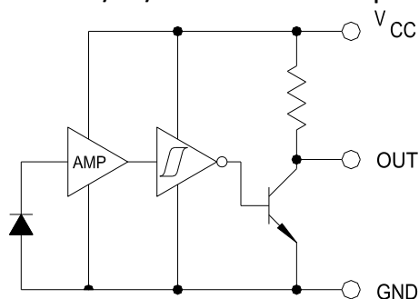
OPB472/482/492 Inverted 10K Pull-Up
