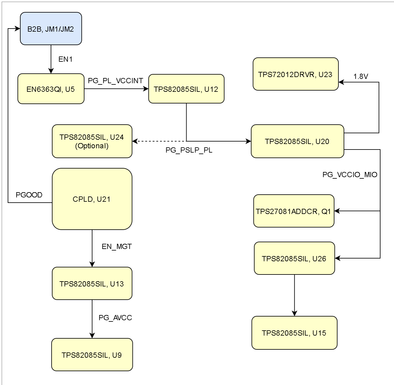
Figure 3: Power Sequency
