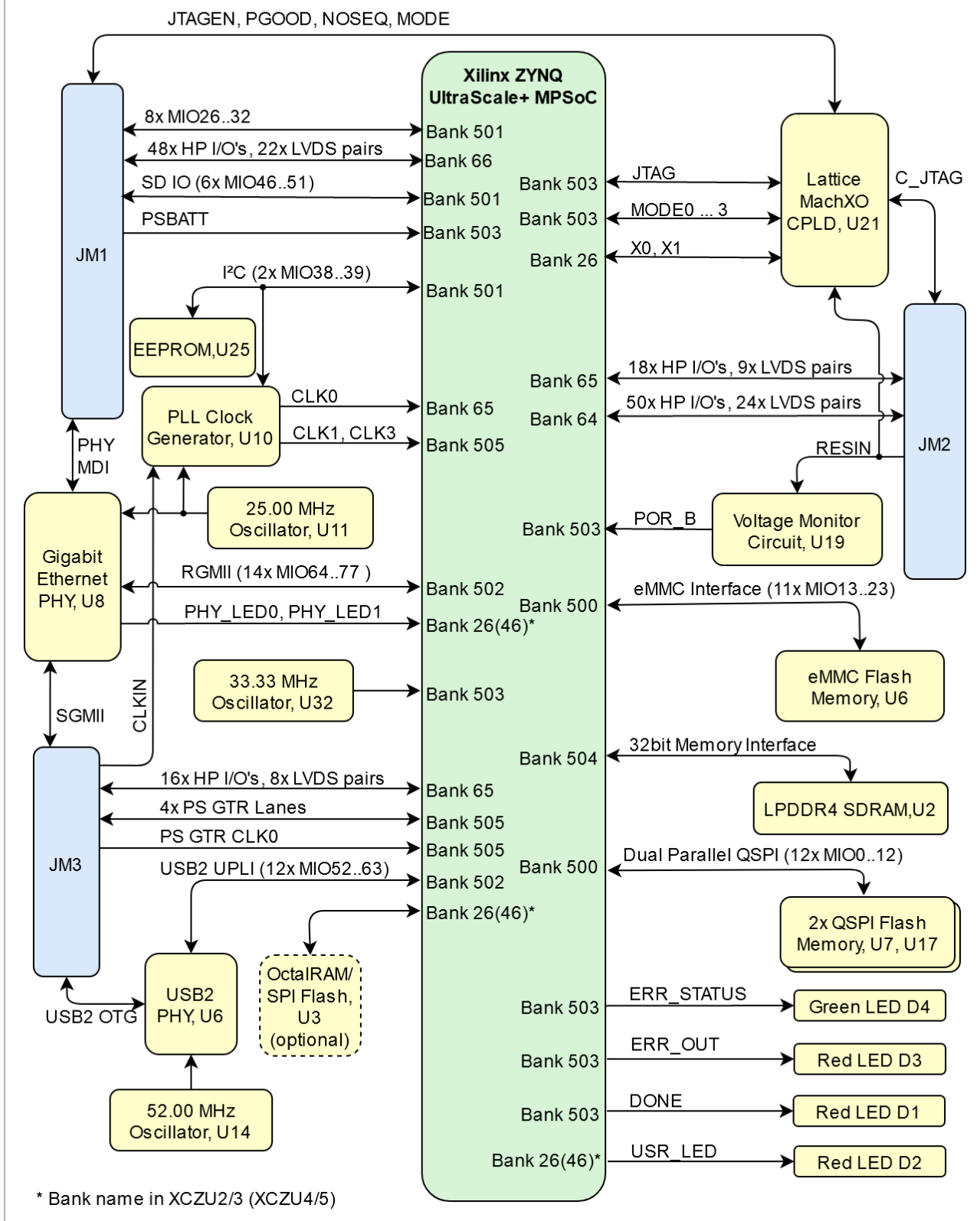
Figure 1: TE0823 block diagram
