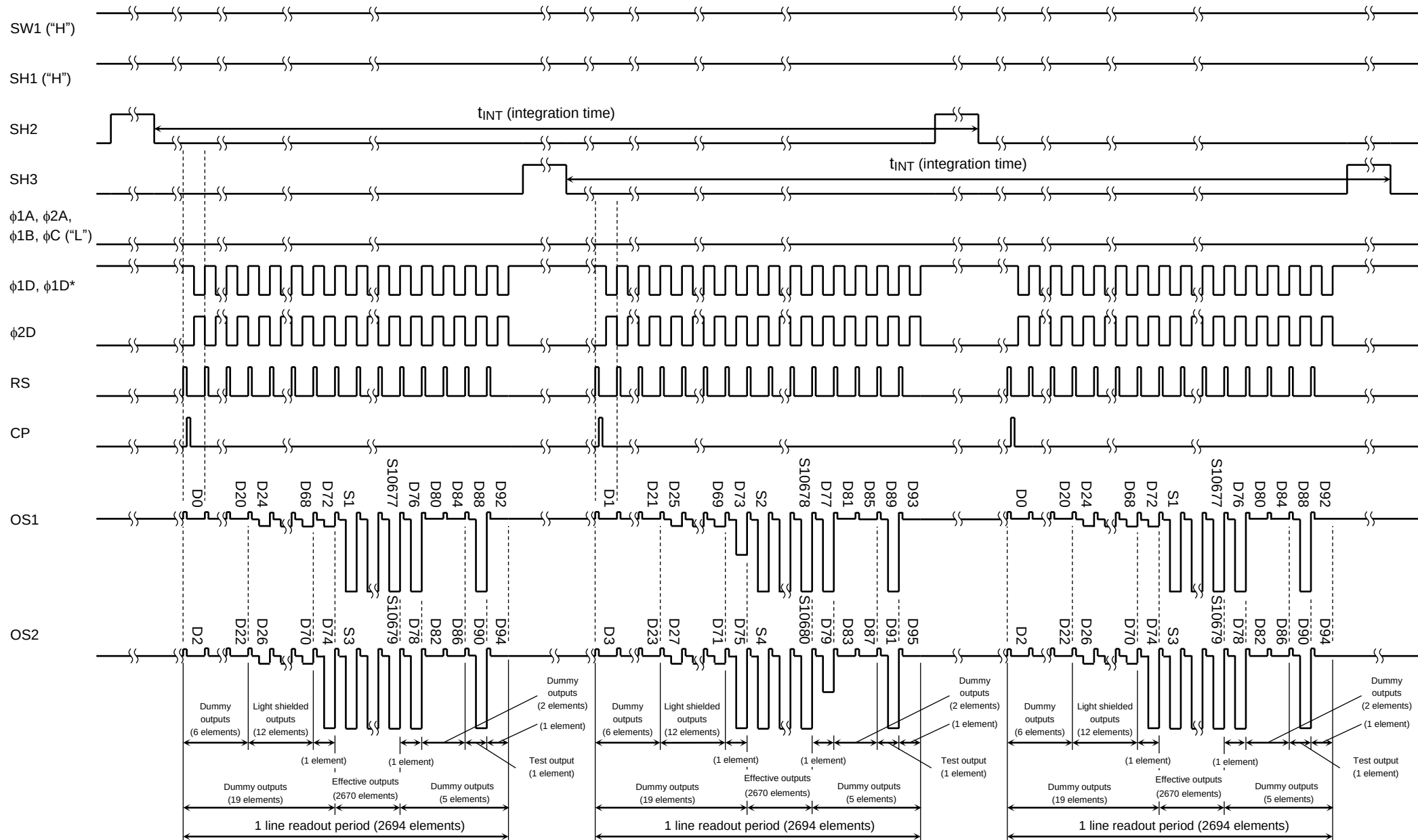
Timing Chart 6: B/W 1200 dpi Mode (Line Clamp Mode)
