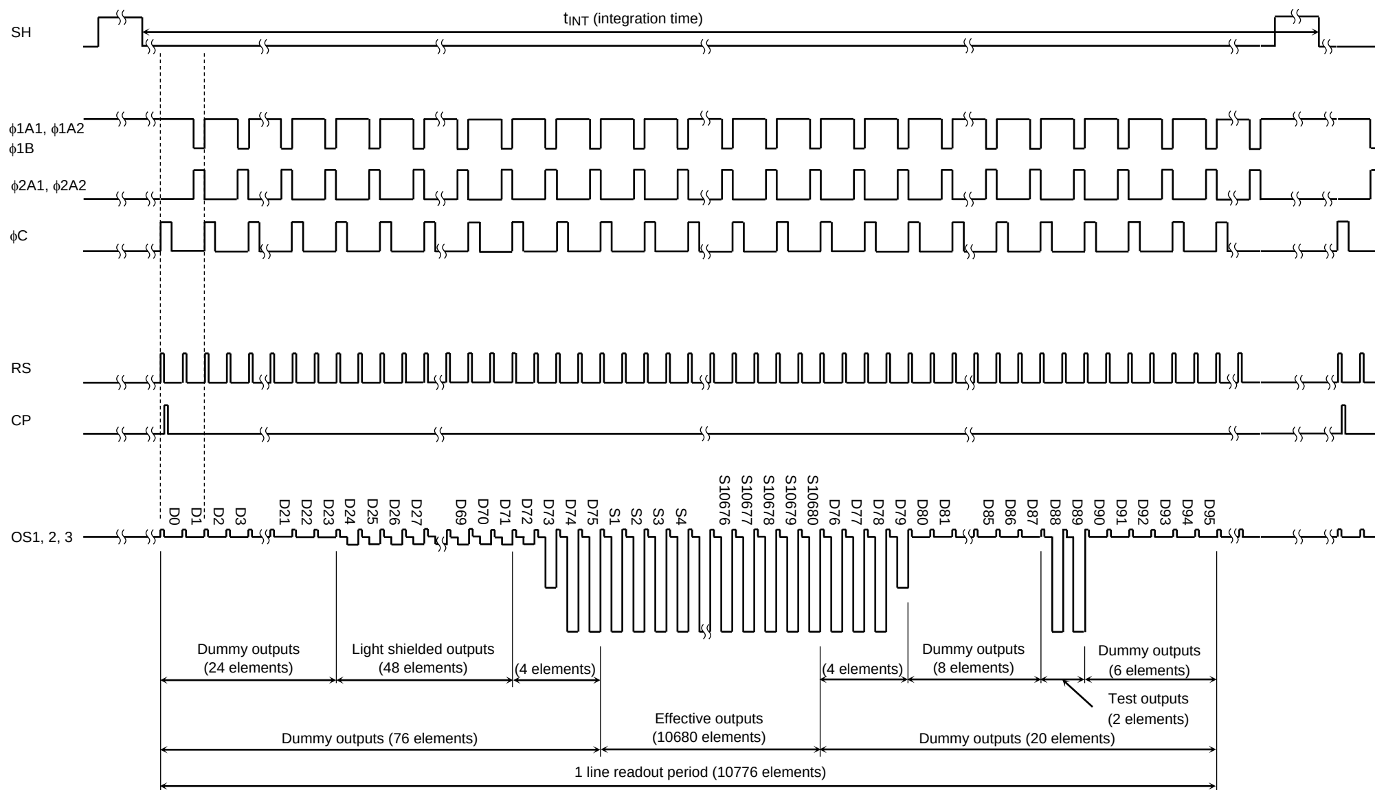
Timing Chart 2: 1200 dpi Mode (Line Clamp Mode)
