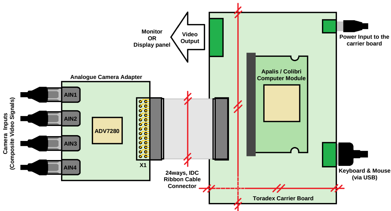
Fig.4 ACA Test Setup - Block Diagram
