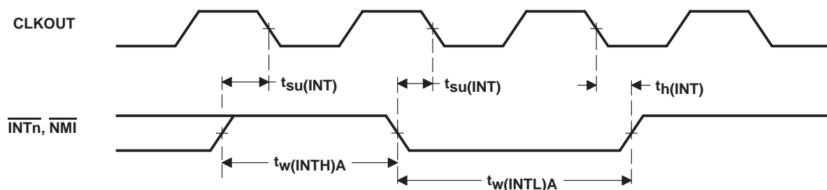
Figure 27. Interrupt Timing
