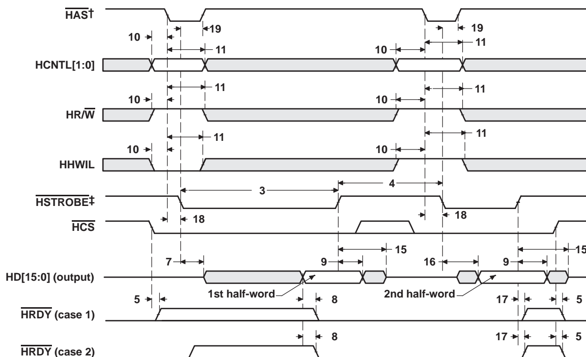
Figure 43. HPI Read Timing (HAS Used)
