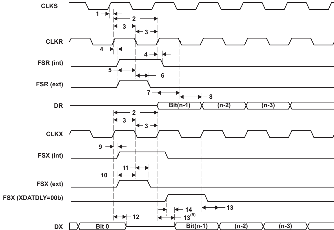
Figure 5-25. McBSP Timing
