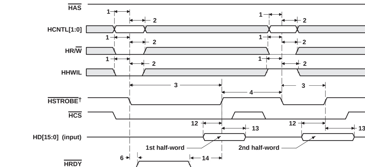
Figure 7–34. HPI16 Write Timing ( \overline{\text{HAS}} Not Used, Tied High)
