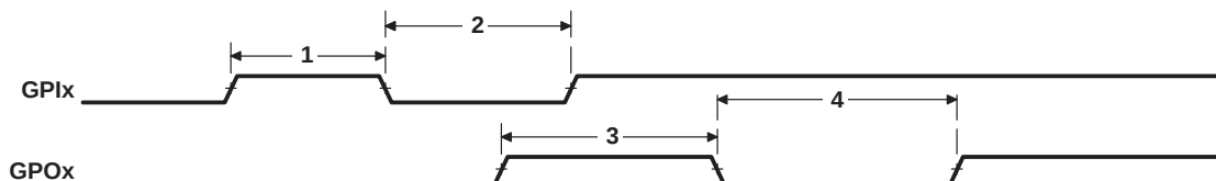
Figure 7–47. GPIO Port Timing
