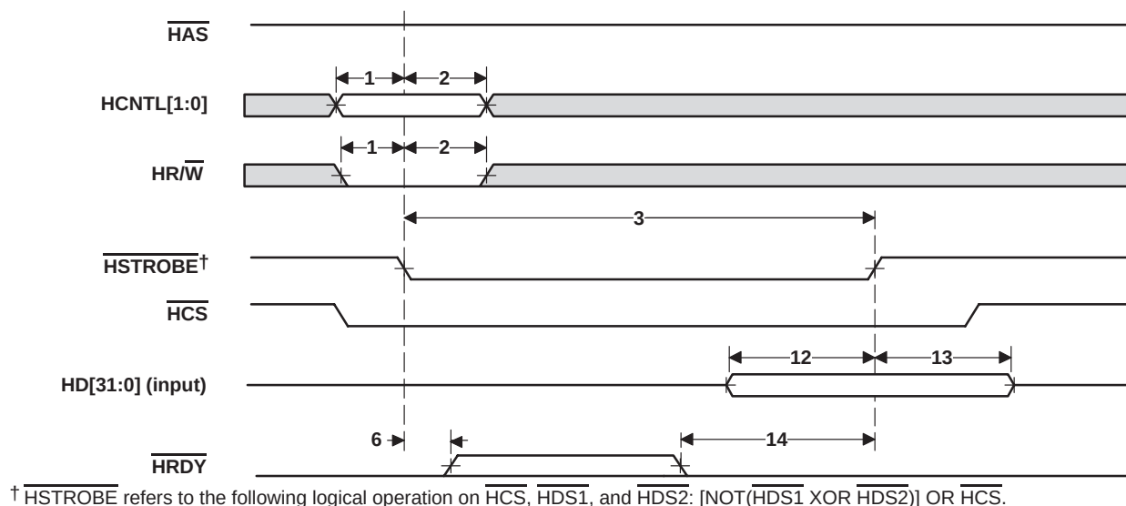
Figure 7–38. HPI32 Write Timing ( \overline{\text{HAS}} Not Used, Tied High)
