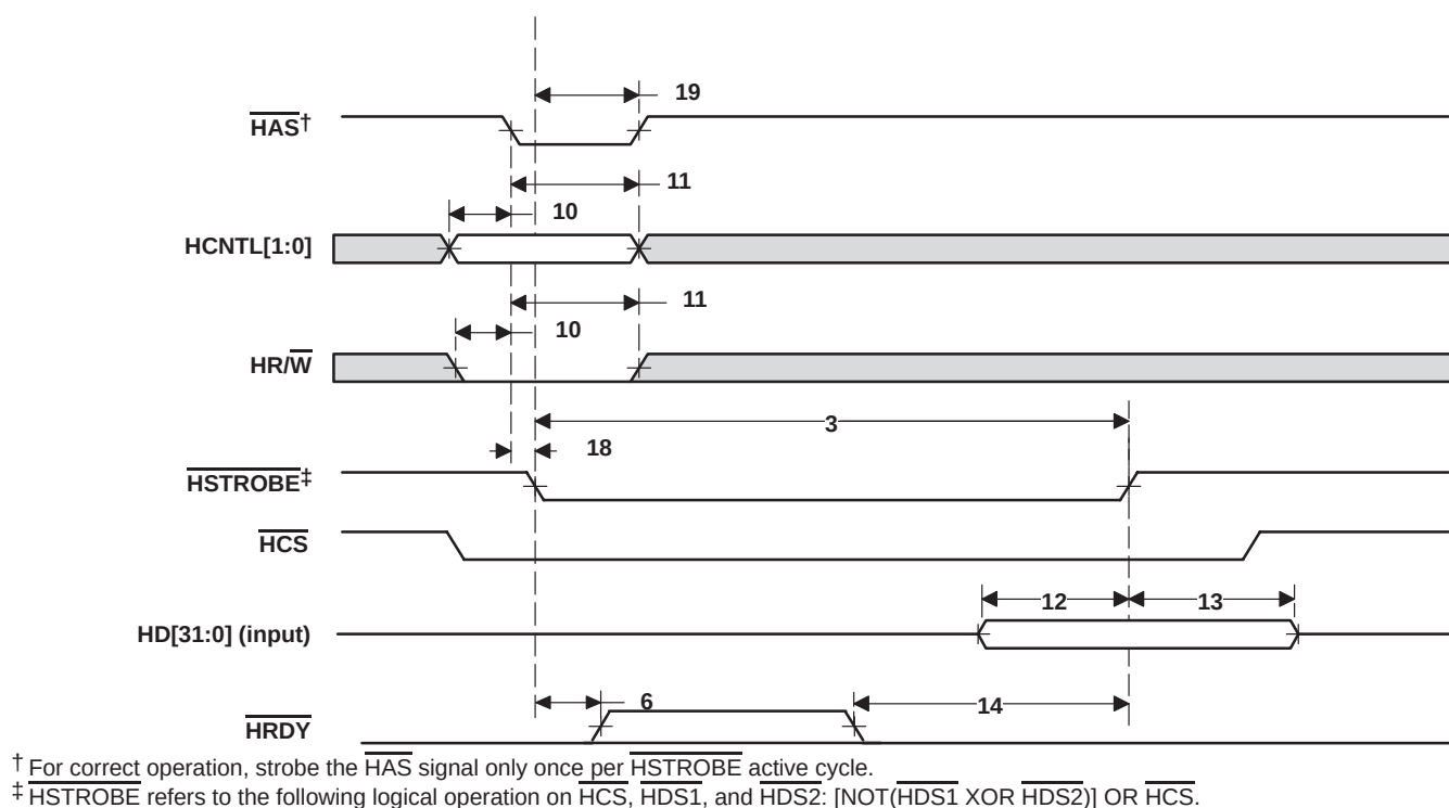
Figure 7–39. HPI32 Write Timing ( \overline{\text{HAS}} Used)
