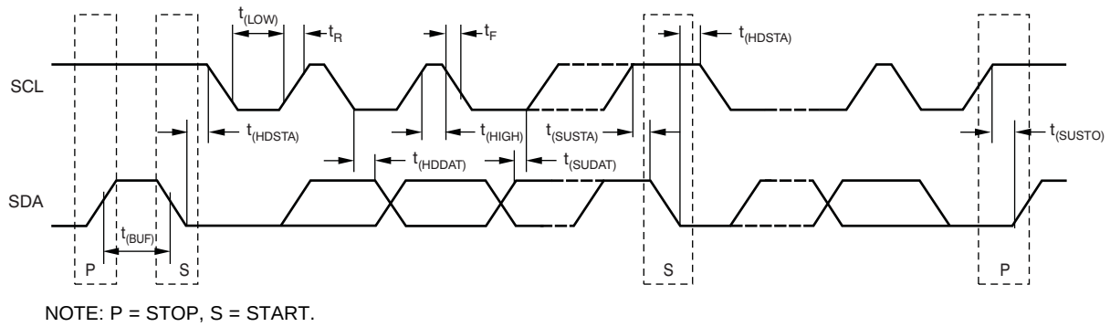
Figure 1. Two-Wire Timing Diagram
