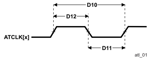
Figure 6-34. ATCLK[x] Timing
