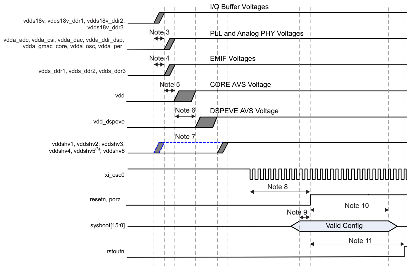
Figure 5-1. Power-Up Sequencing
