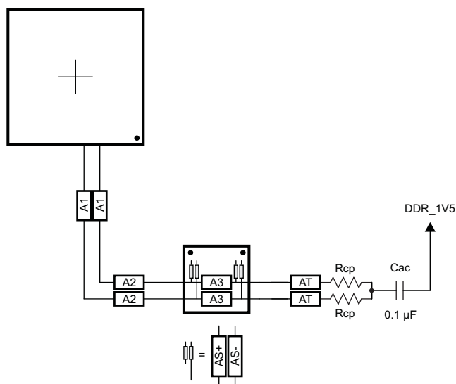
Figure 8-53. CK Routing for Two Mirrored DDR3 Devices
