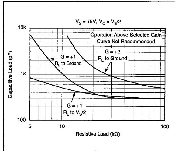
FIGURE 5. Stability—Capacitive Load vs Resistive Load.
