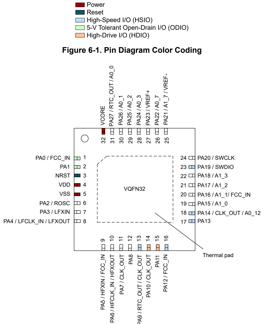
Figure 6-2. 32-Pin RHB (VQFN) (Top View)
