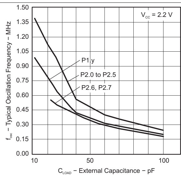
Figure 5-11. Typical Oscillating Frequency vs Load Capacitance One output active at a time.
