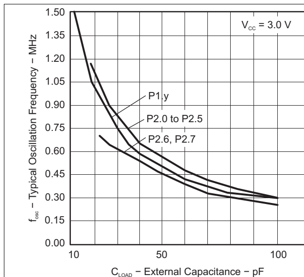
Figure 5-10. Typical Oscillating Frequency vs Load Capacitance One output active at a time.
