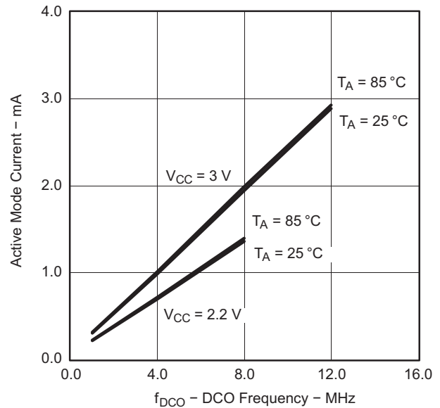
Figure 5-3. Active Mode Current vs DCO Frequency
