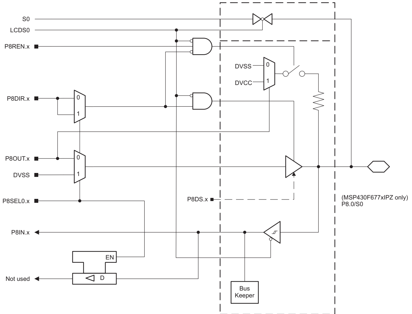
Figure 6-30. Port P8 (P8.0) Diagram (MSP430F677xLPZ Only)
