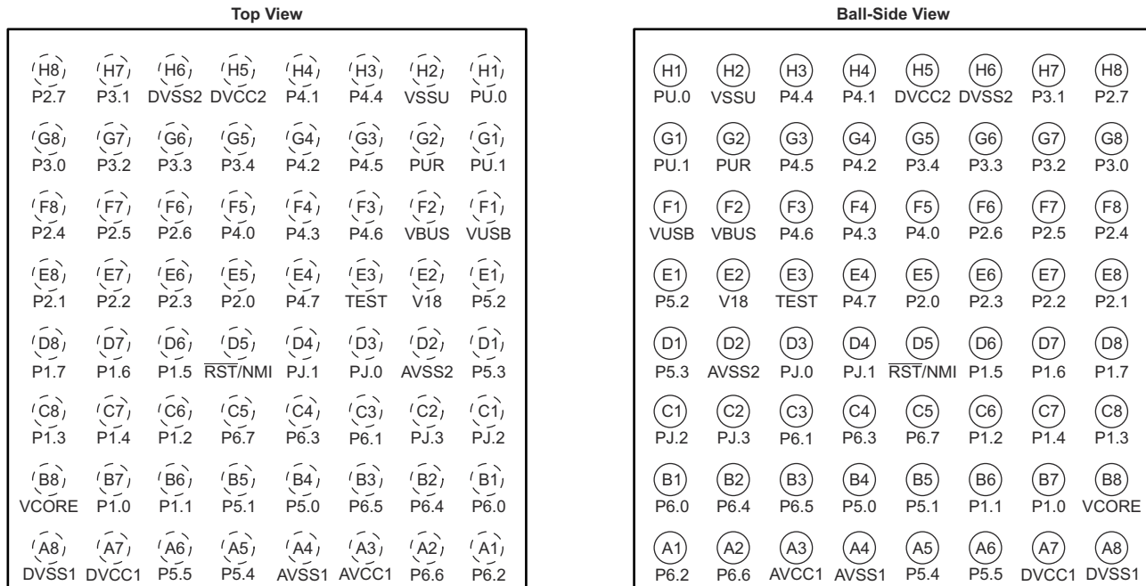
Figure 7-6. 64-Pin YFF Package – MSP430F5528IYFF
